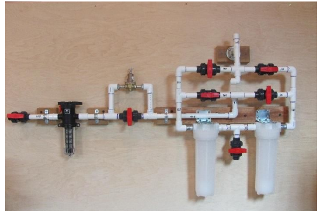
BACKFLUSH RIGHT FILTER POSITION
